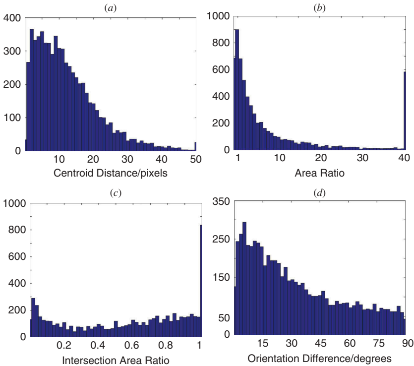
Figure 6. Histograms of four attributes including (a) centroid distance, (b) area ratio, (c) intersection area ratio, and (d) orientation difference for satellite product PERSIANN in the summer of 2008. In the centroid distance histogram, one pixel unit is approximately 25 km in length.
